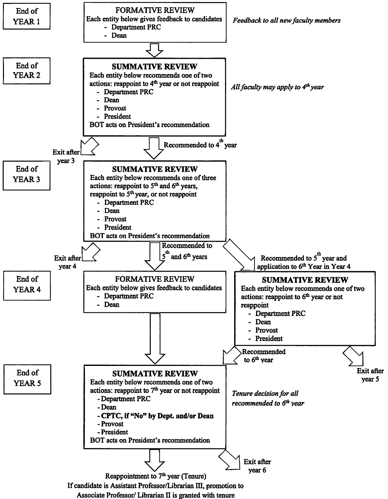
Figure 1 - REAPPOINTMENT PROCESS
